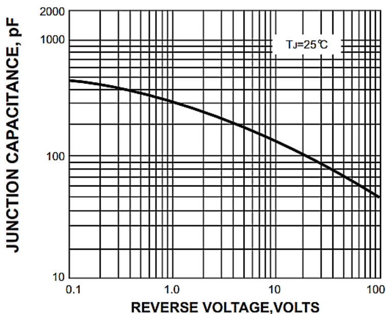
FIG. 5-TYPICAL JUNCTION CAPACITANCE
