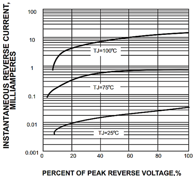
FIG. 4-TYPICAL REVERSE CHARACTERISTICS
