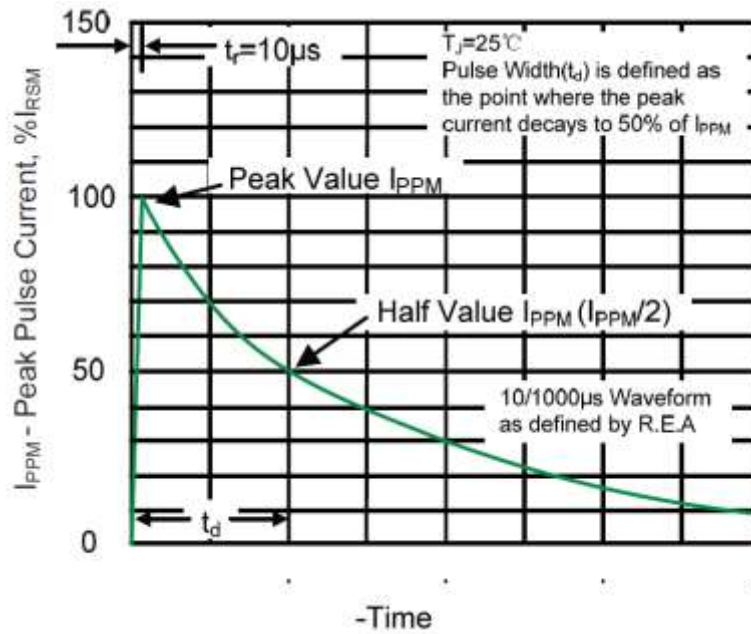
Figure 3. Pulse Waveform
