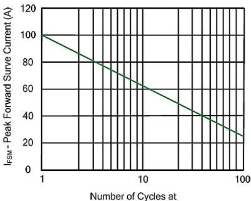
Figure 6. Maximum Non-Repetitive Forward Surge Current Uni-Directional Only
