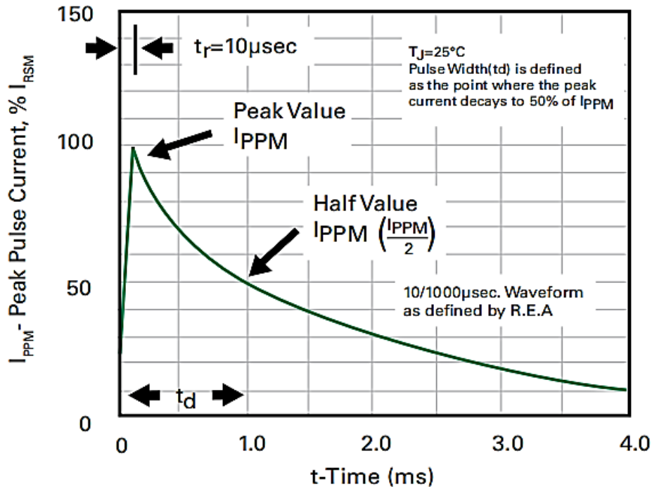
Figure 3. Pulse Waveform
