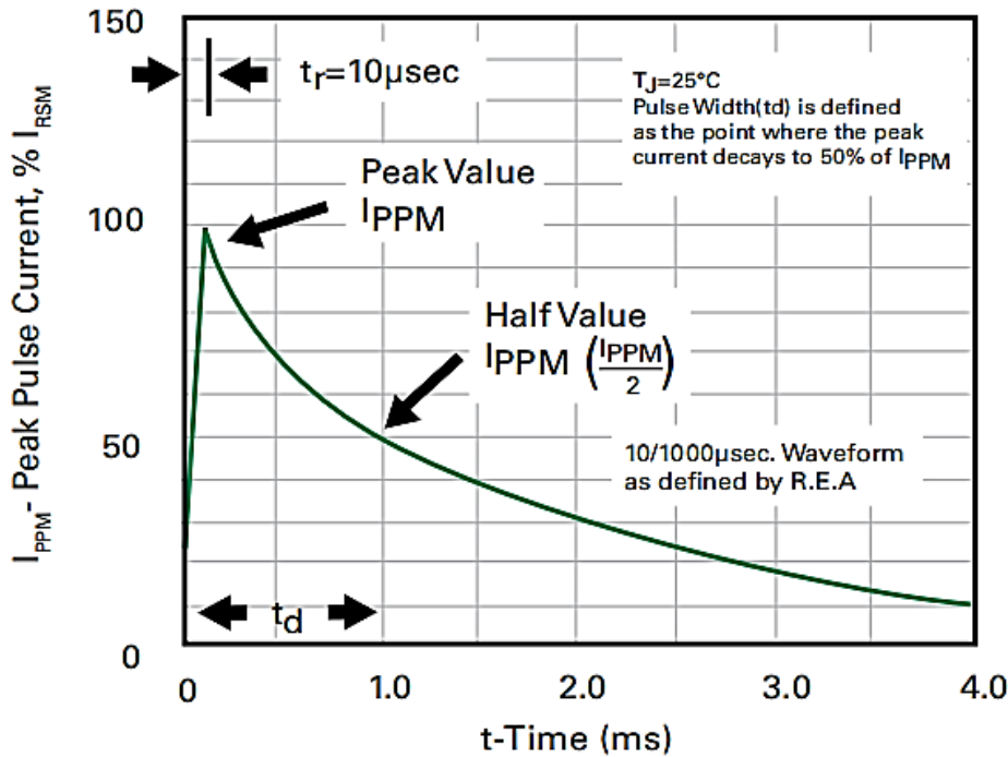
Figure 3. Pulse Waveform
