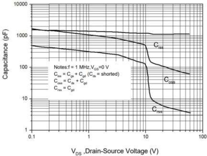
Figure 7. Capacitance Characteristics
