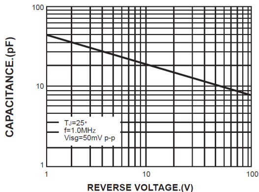
FIG. 3- TYPICAL JUNCTION CAPACITANCE PER BRIDGE ELEMENT
